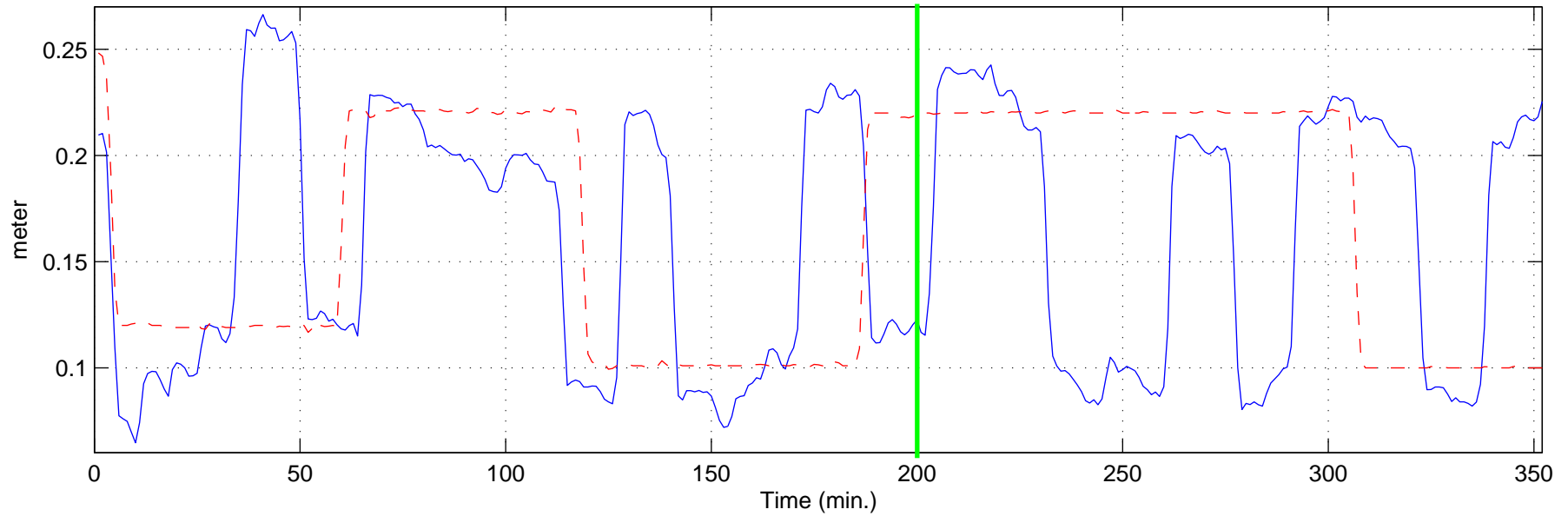
Head over gate 9 (solid) and gate 10 position (dashed)
