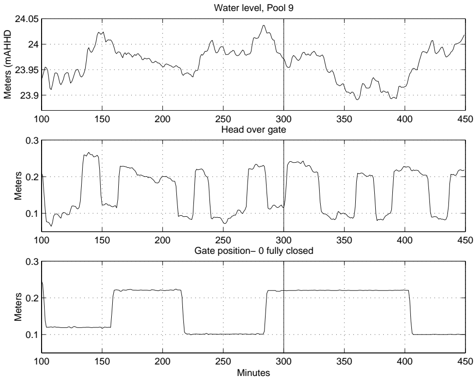
Figure 2: Water level, head over upstream gate and downstream gate position.
